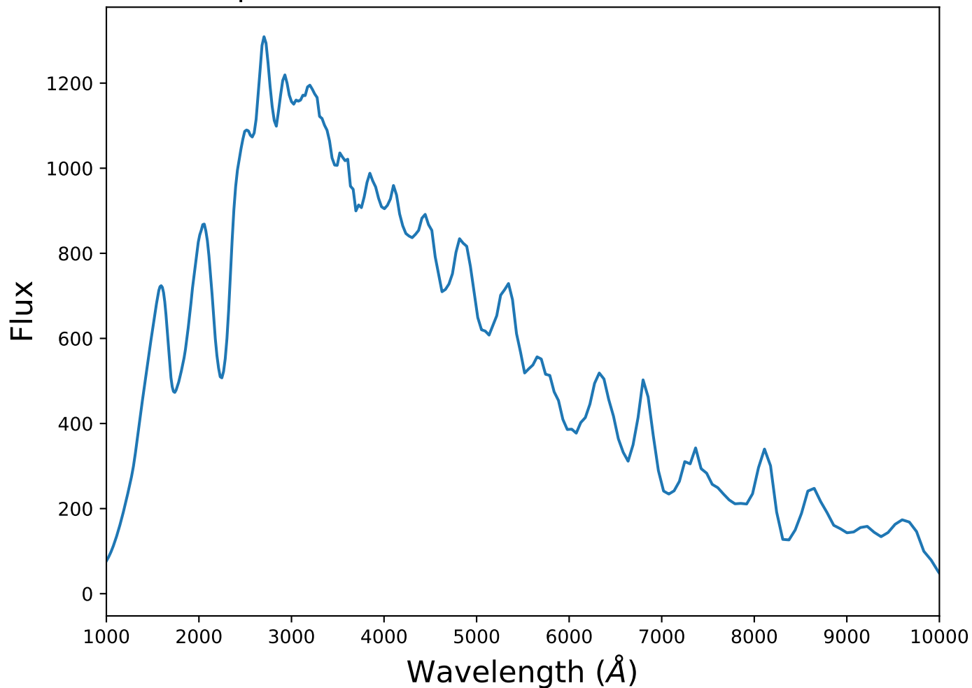
Spectrum 3 for transient SLSN at z=2.70
